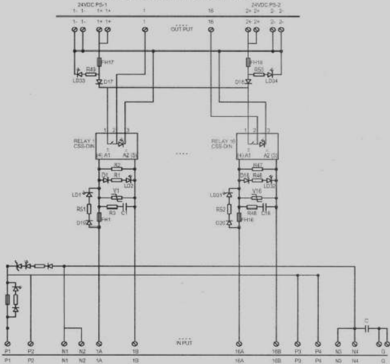
16 CHANNEL INPUT RELAY MODULE CIRCUIT DIAGRAM
